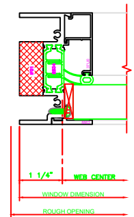
403 JAMB 325 PROJECT OUT \ FIXED
